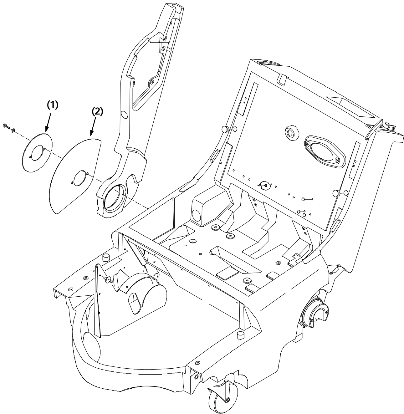
FIG. 1 - Skirt And Retainer Assembly BILL OF MATERIALS FOR DIRT SHIELD KIT 80105
