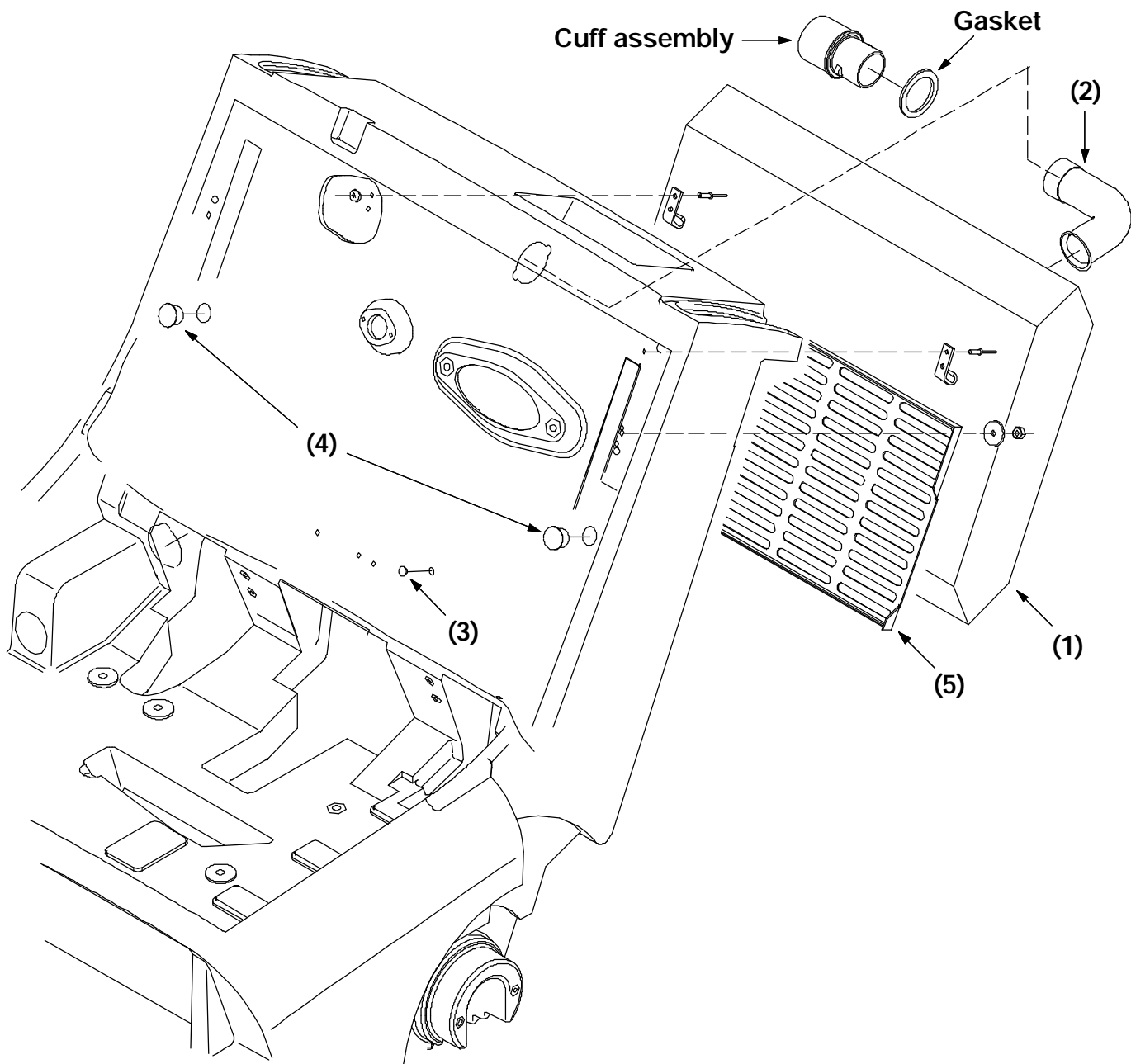
FIG. 1 - Filter Bag Assembly BILL OF MATERIALS FOR FILTER BAG KIT #80978
