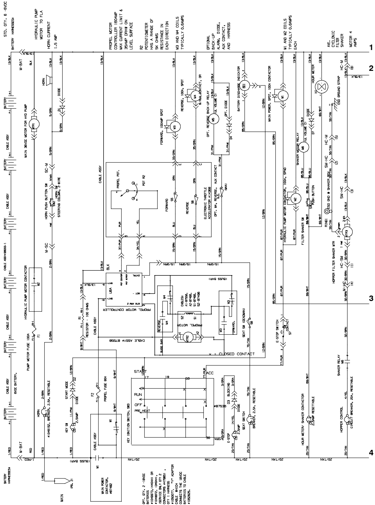
ELECTRICAL SCHEMATIC FIG 1
