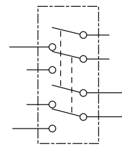
DPDT Switch
