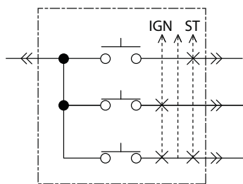
Key Switch
