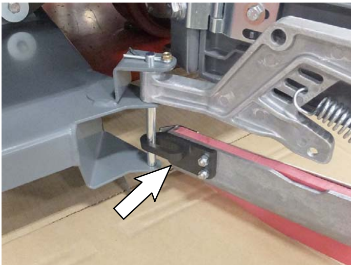
p/n 1201455 Block, Squeegee, Guide, RH p/n 1200689 Block, Squeegee, Guide, LH
