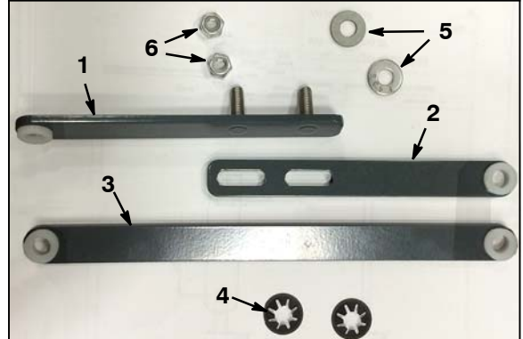
Upgrade Kit 9013049 Contents
