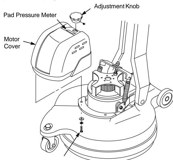
Motor Cover Screws (4)
