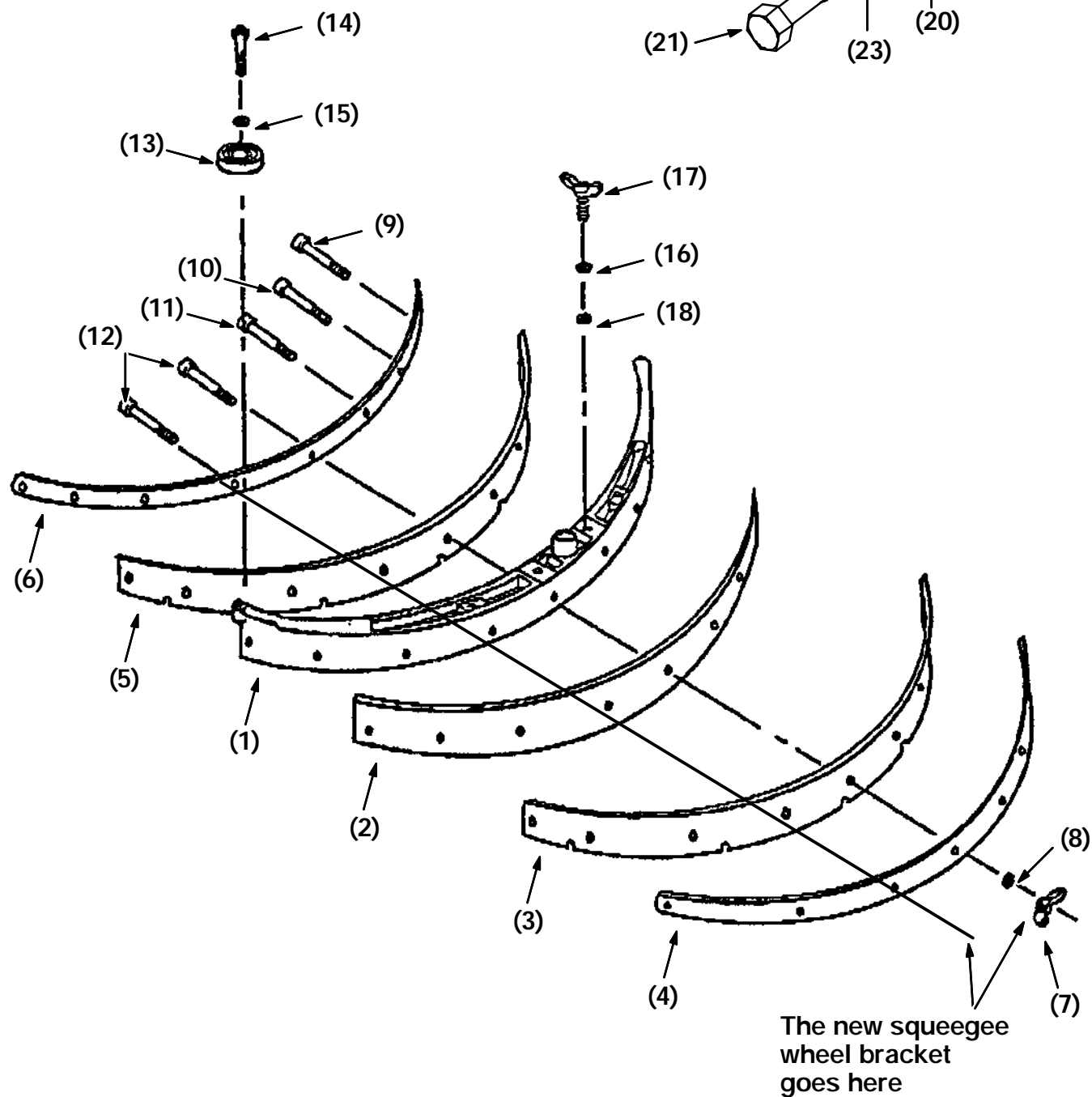
FIG. 1 - New Rear Squeegee Assembly
