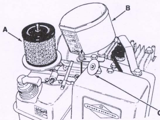
Fig. 1 - AIR CLEANER ASSEMBLY
