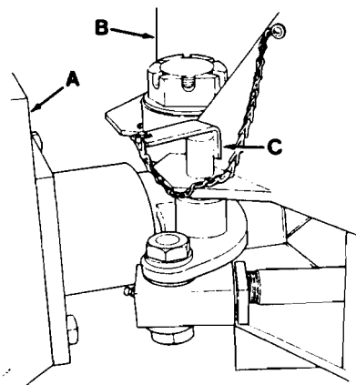
A. Machine Trailer Section B. Machine Tractor Section C. Pivot Lock Pin
