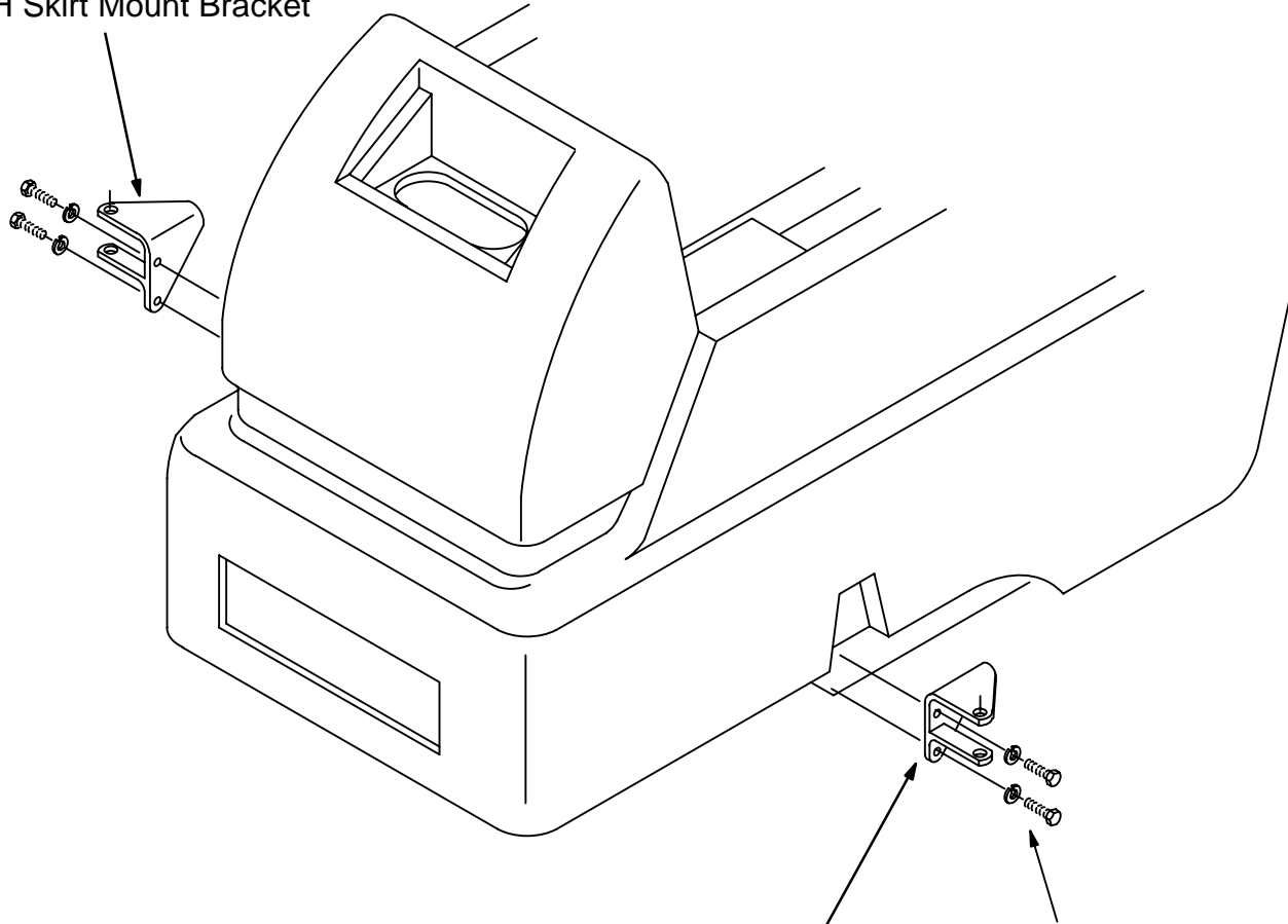
LH Skirt Mount Bracket
