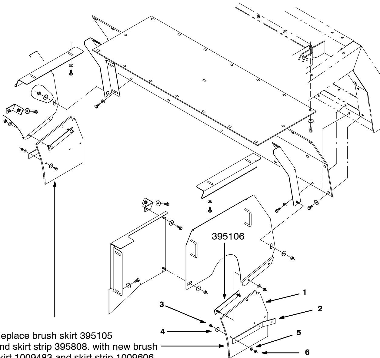
FIG. 1 - Brush Skirt Replacement
