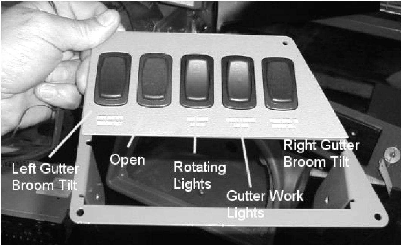
FIG. 3 - Work Light Switch Installation
