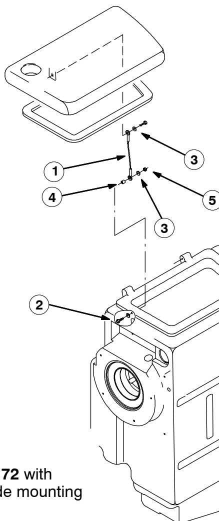
FIG. 1 - Recovery Tank Cable Installation
