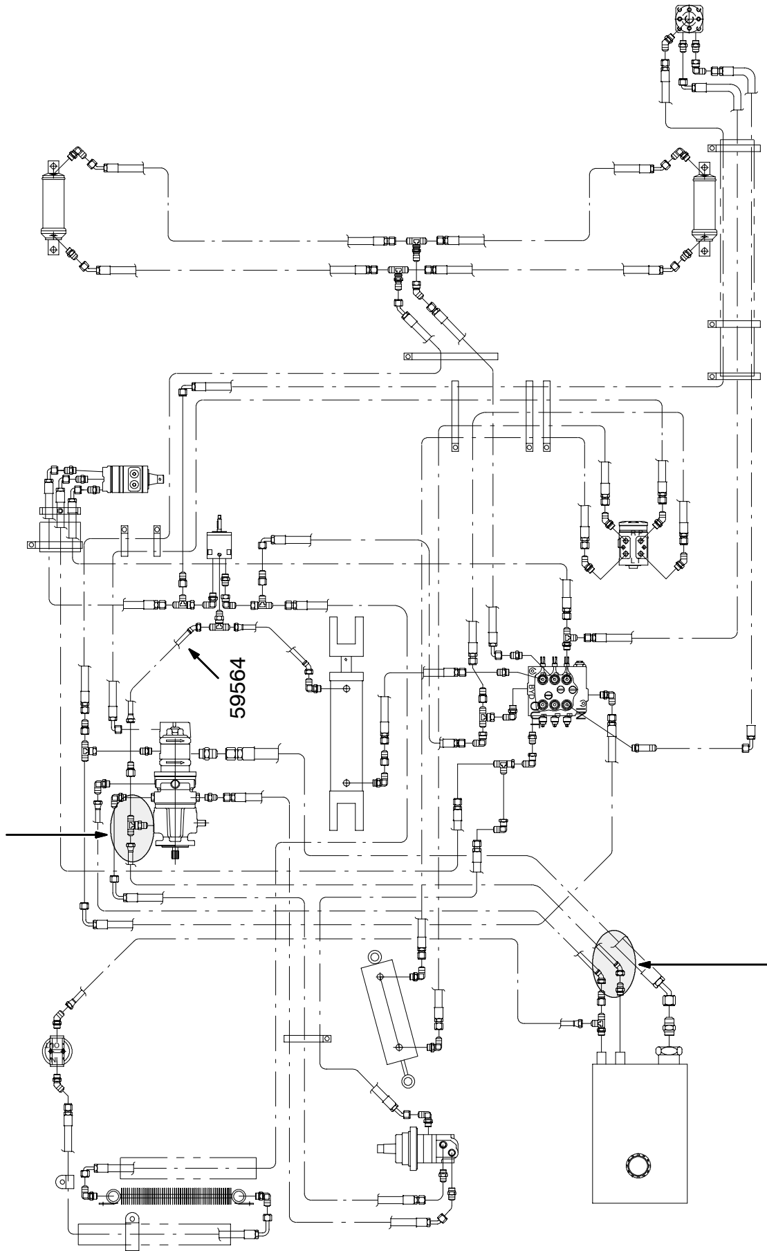
FIG. 1 - HYDRAULIC HOSE GROUP
