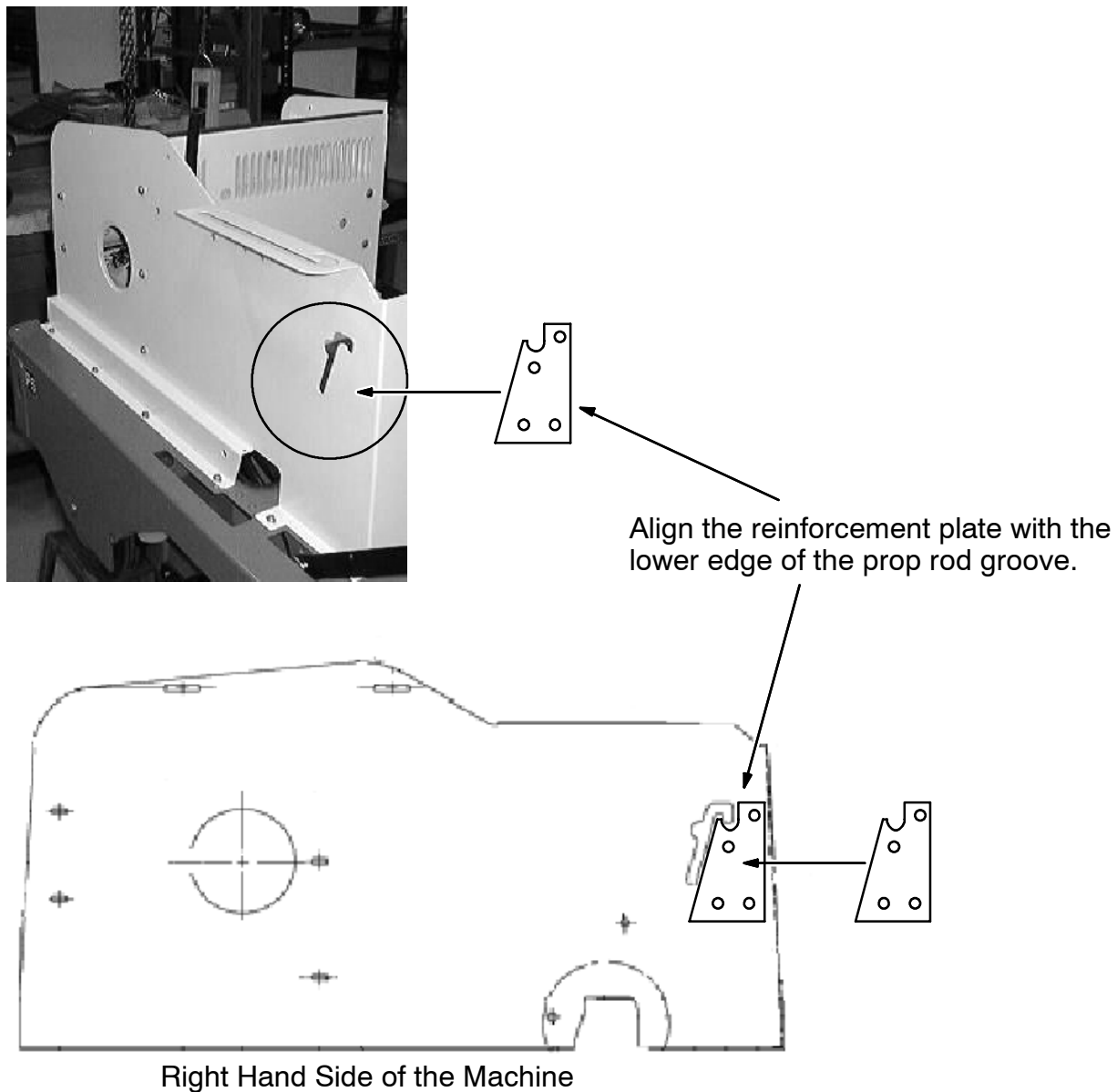
FIG. 1 - Reinforcement Plate Installation
