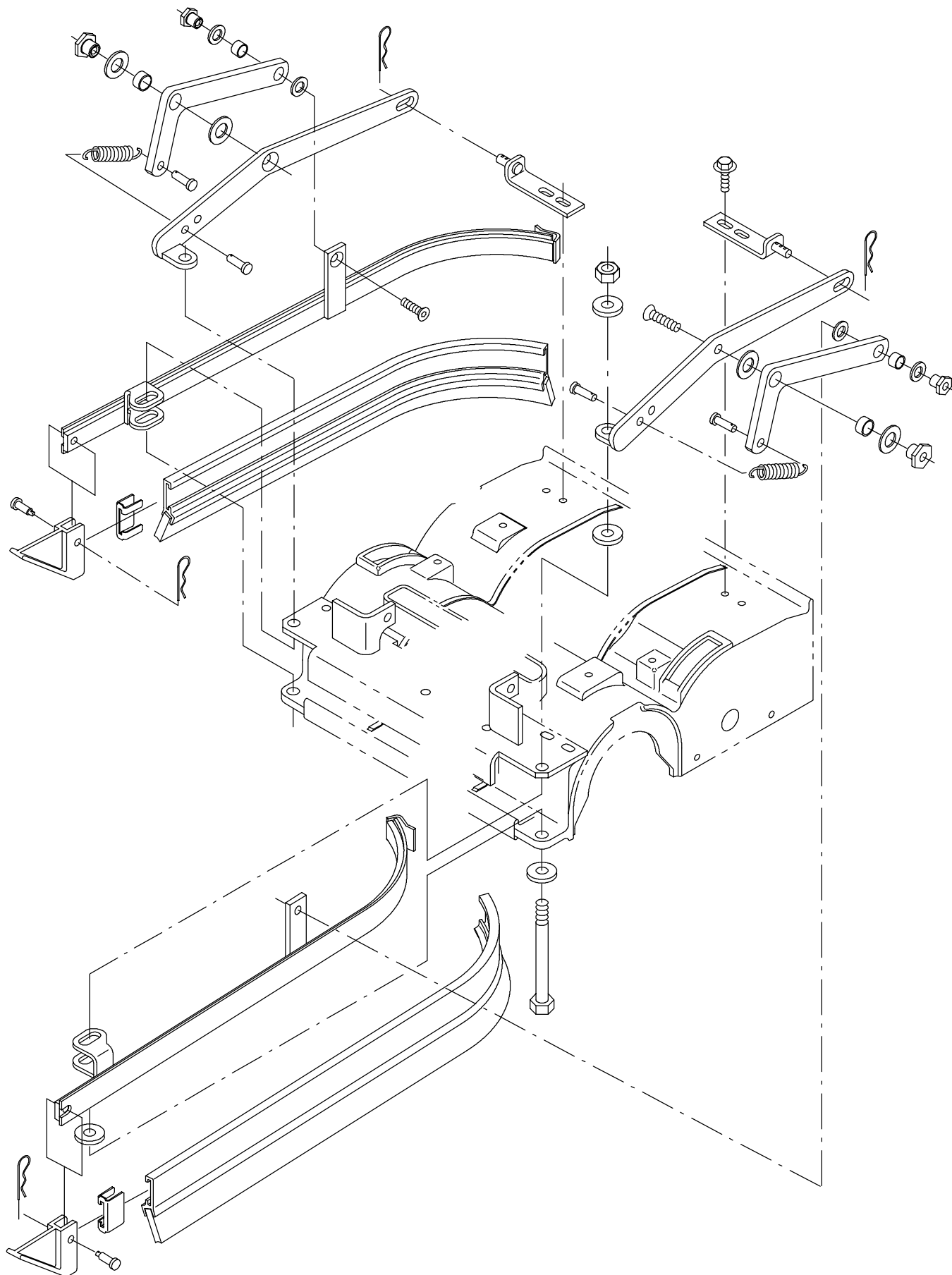
FIG. 5 - Cylindrical Scrub Head Squeegee Group
