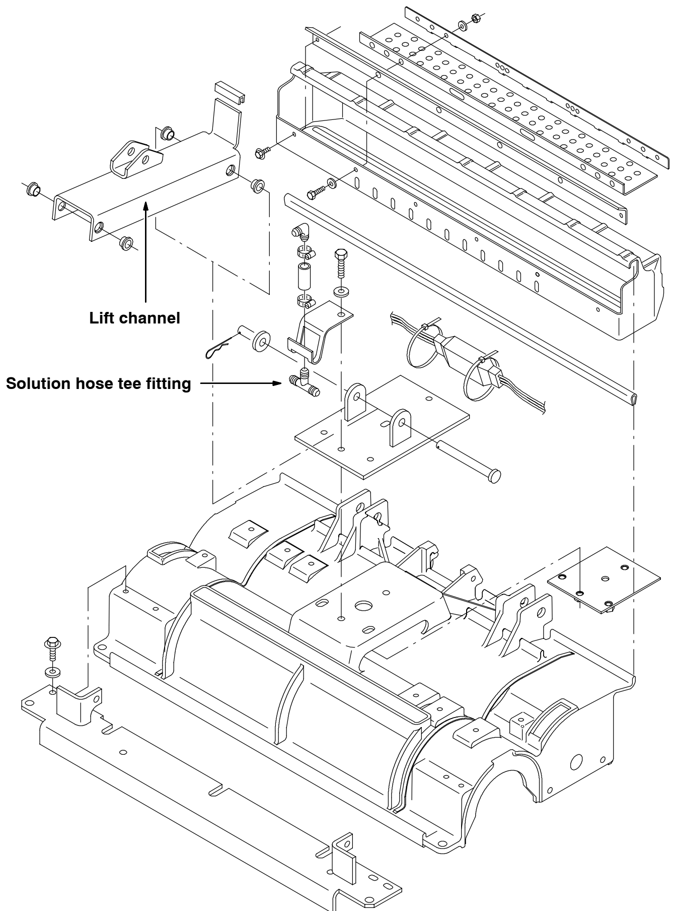
FIG. 4 - Cylindrical Scrub Head Frame Group
