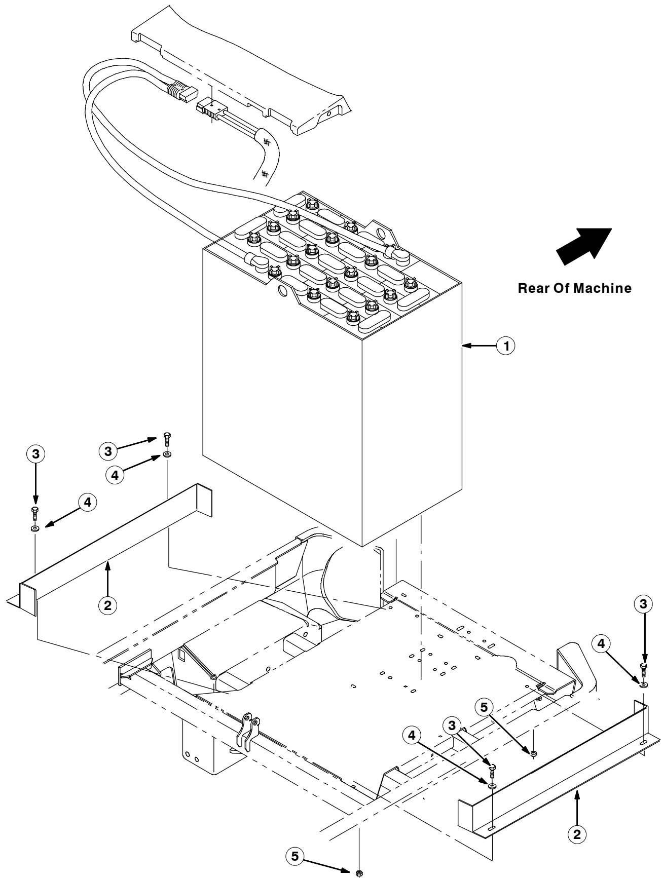
FIG. 2 - BATTERY KIT, 8300 (36VDC, 380AH) INSTALLATION
