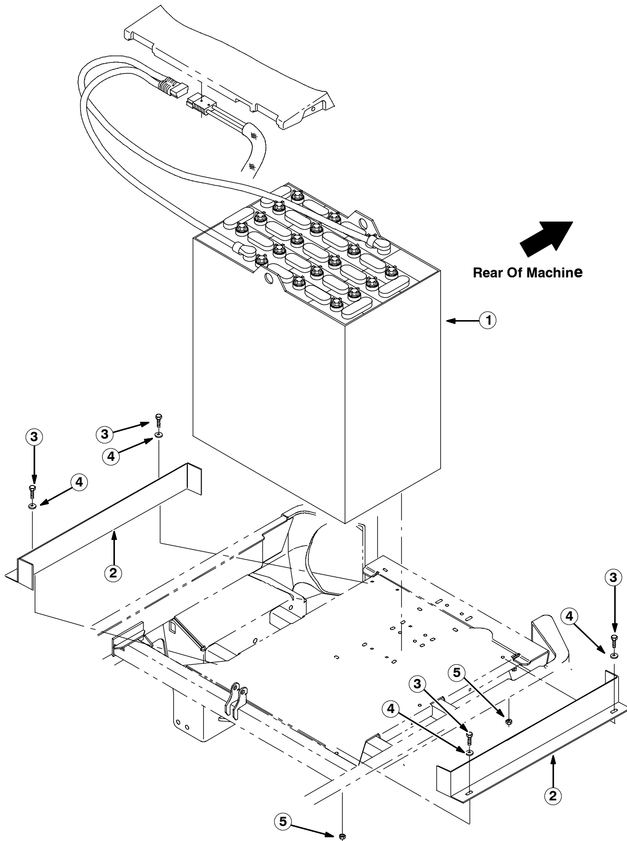
FIG. 1 - BATTERY KIT, 7300 (36VDC, 380AH) INSTALLATION
