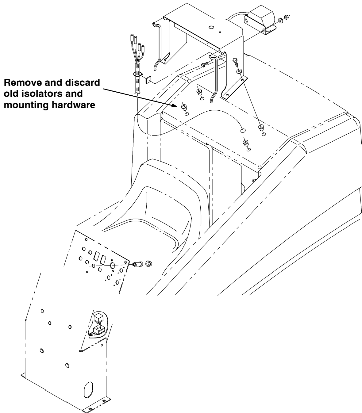
FIG. 2 - MOUNTING BRACKET ISOLATOR NUT LOCATIONS
