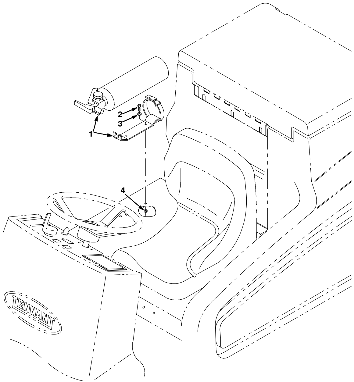
FIG. 2 - FIRE EXTINGUISHER KIT INSTALLATION
