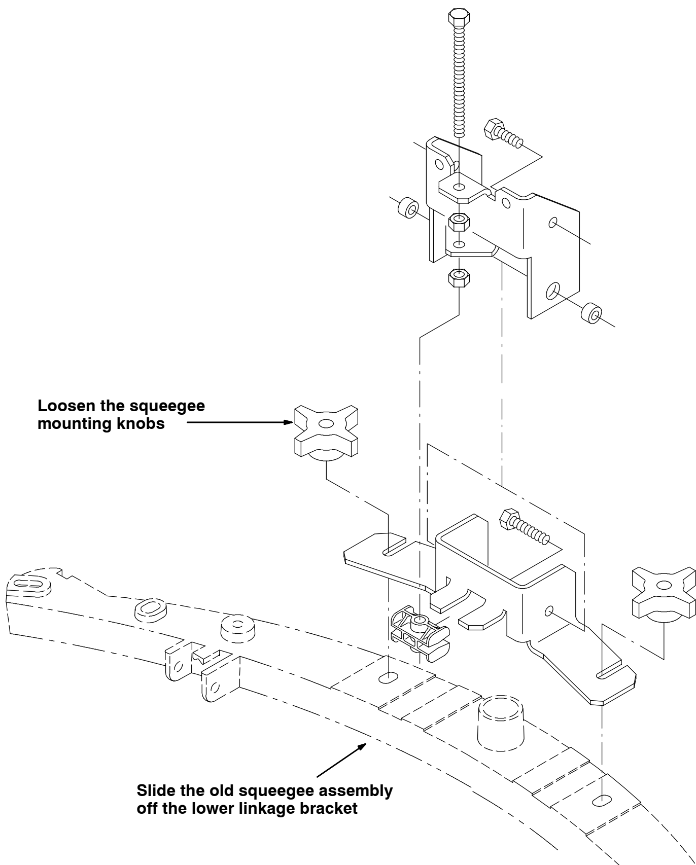
FIG. 1 - Squeegee Linkage Group
