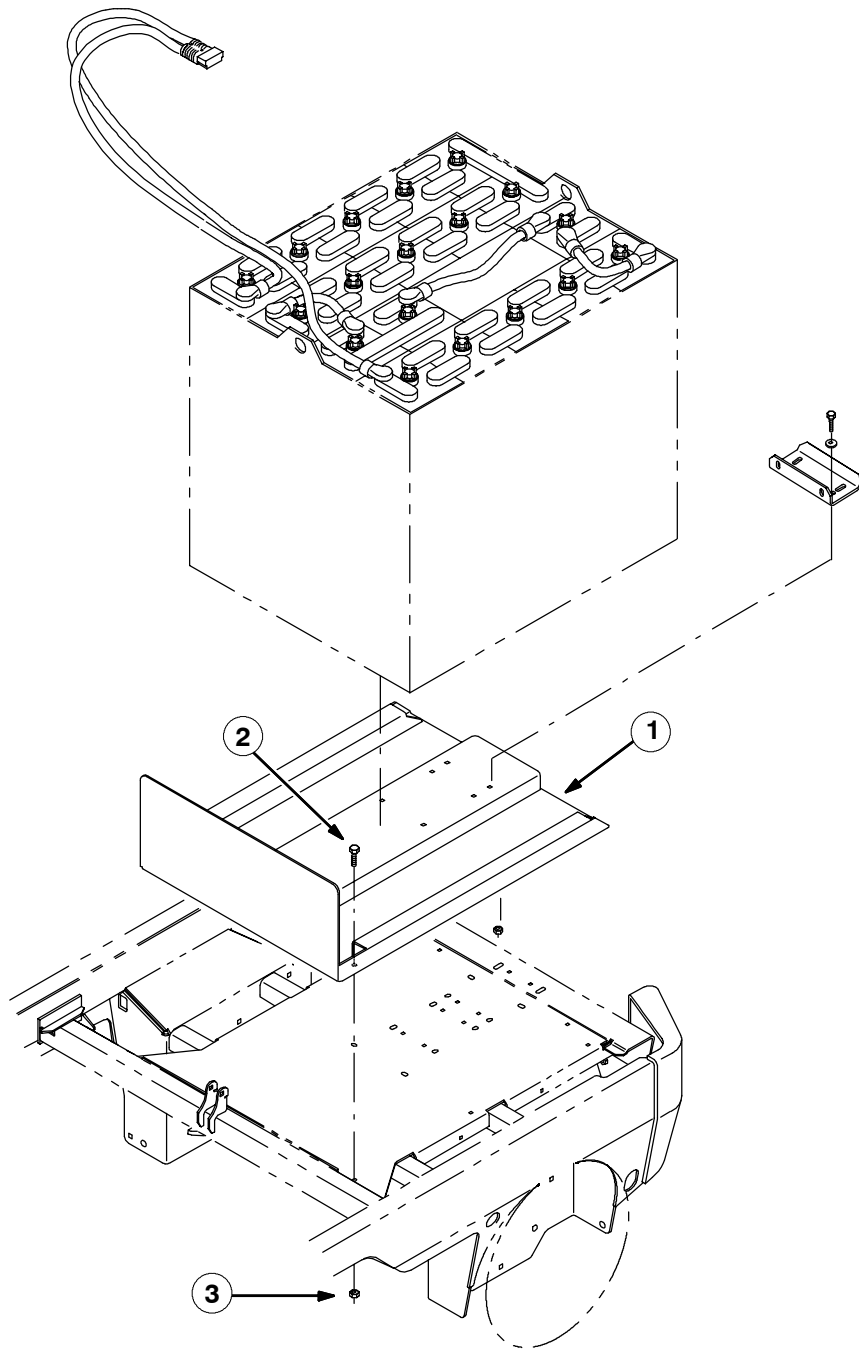
FIG. 1 - FORK LIFT BATTERY KIT INSTALLATION
