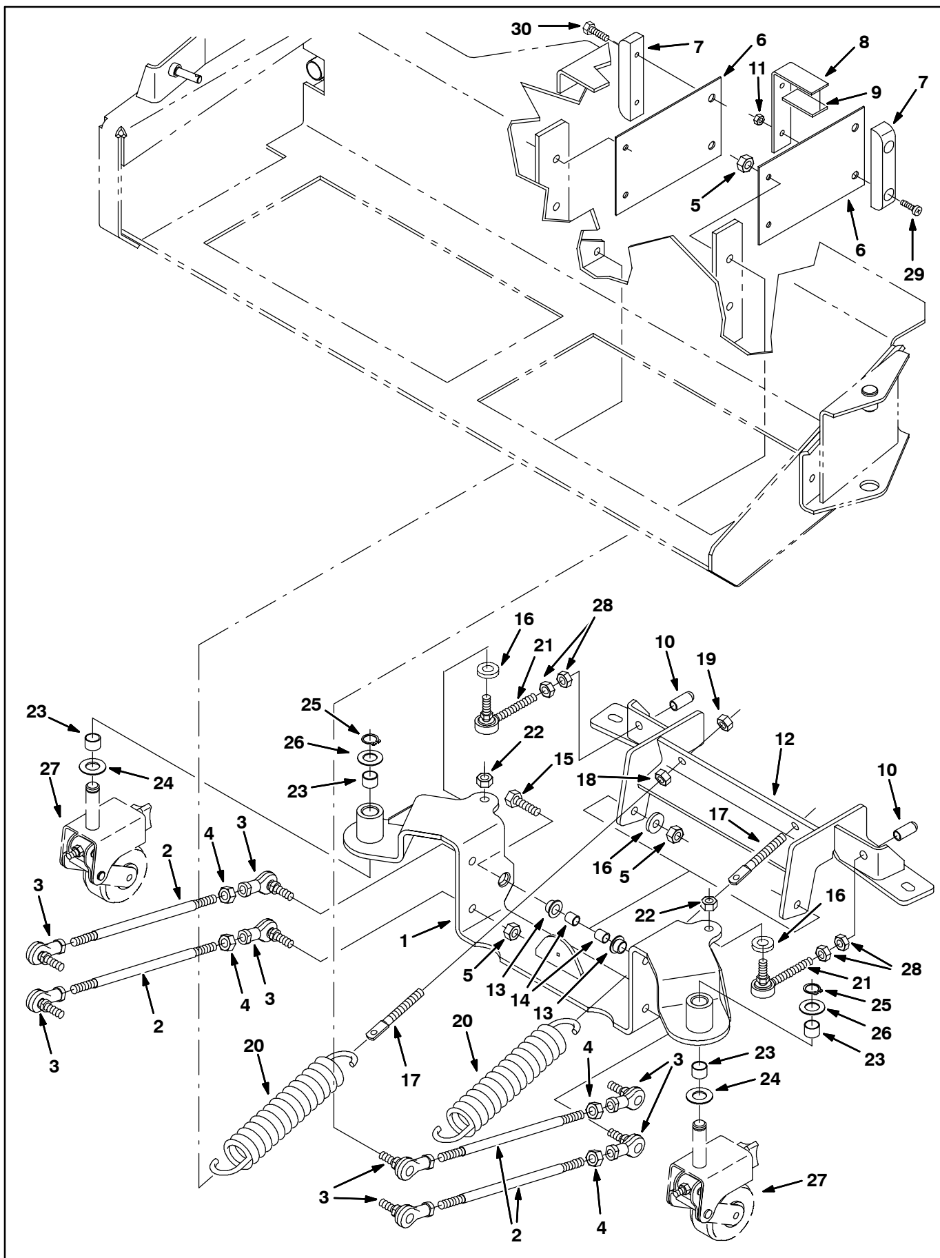
FIG. 1 - REAR SQUEEGEE LINKAGE GROUP
