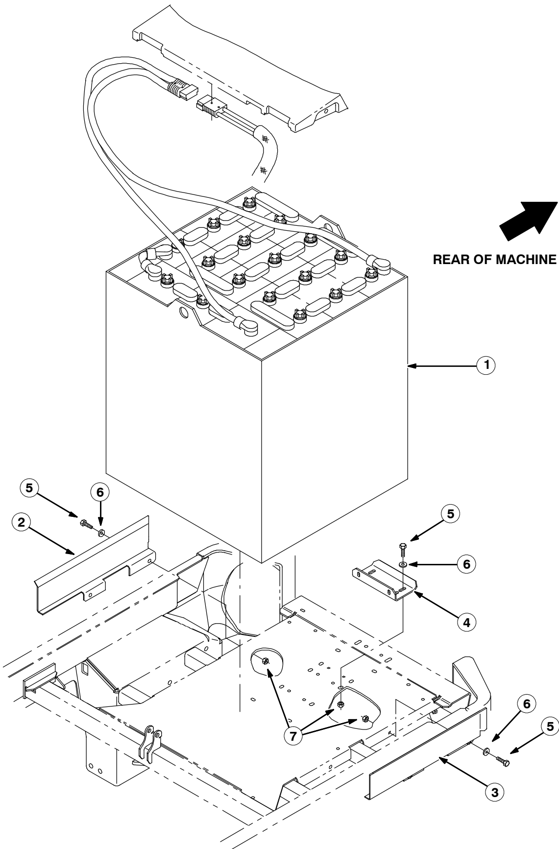
FIG. 1 - BATTERY KIT (750 AH, WET)
