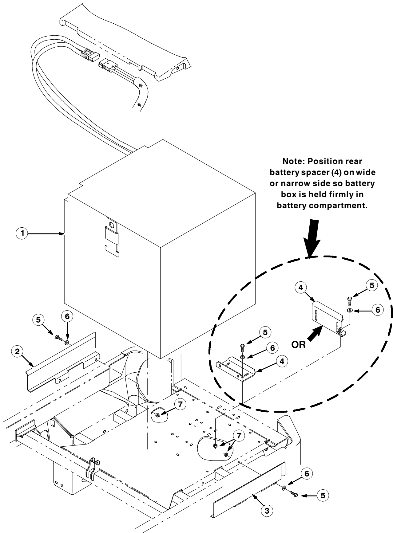
FIG. 1 - 600 AH BATTERY KIT
