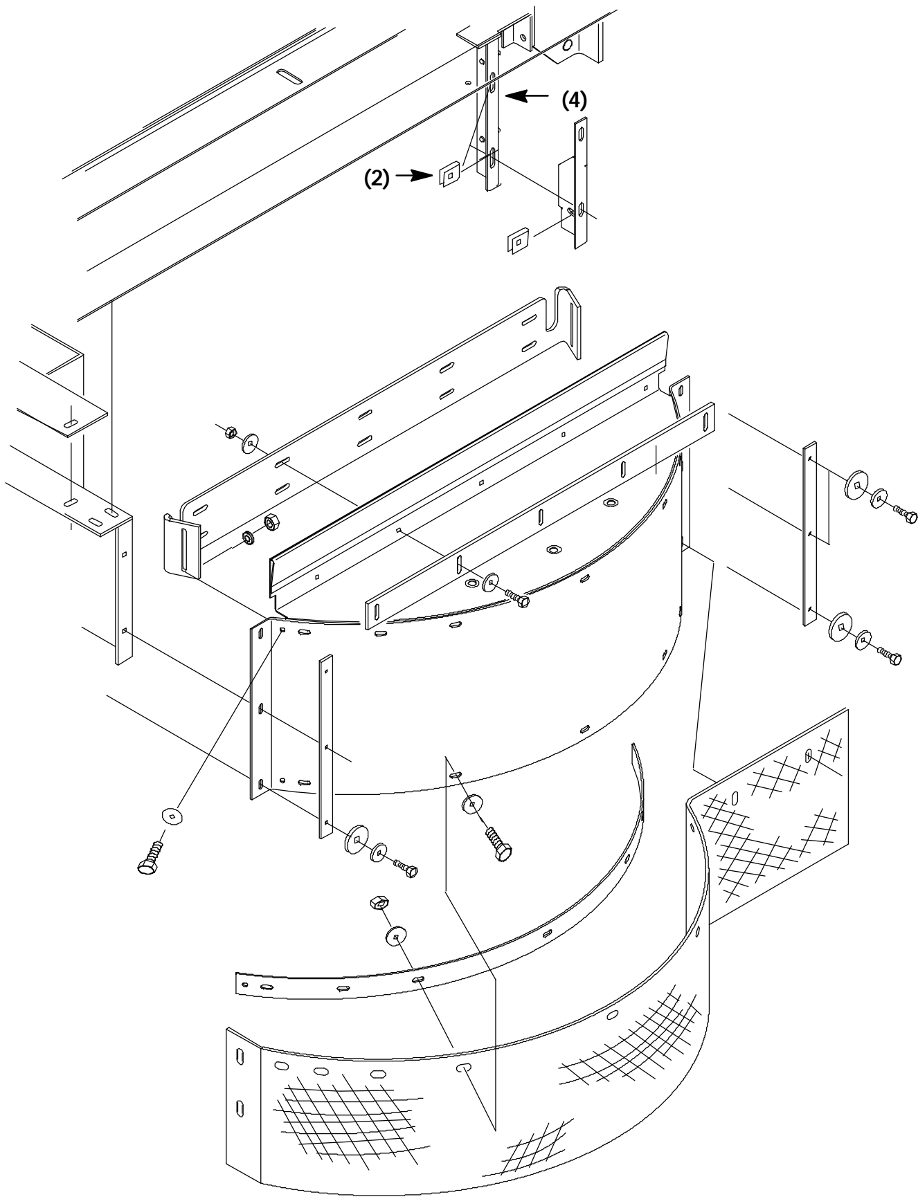
FIG. 3 - Left Side Dry Dust control assembly
