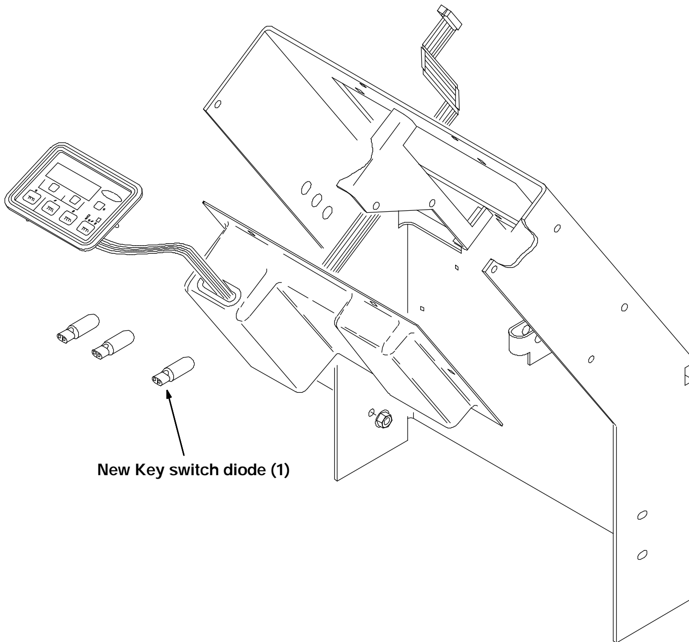
FIG. 1 - Diode Assembly
