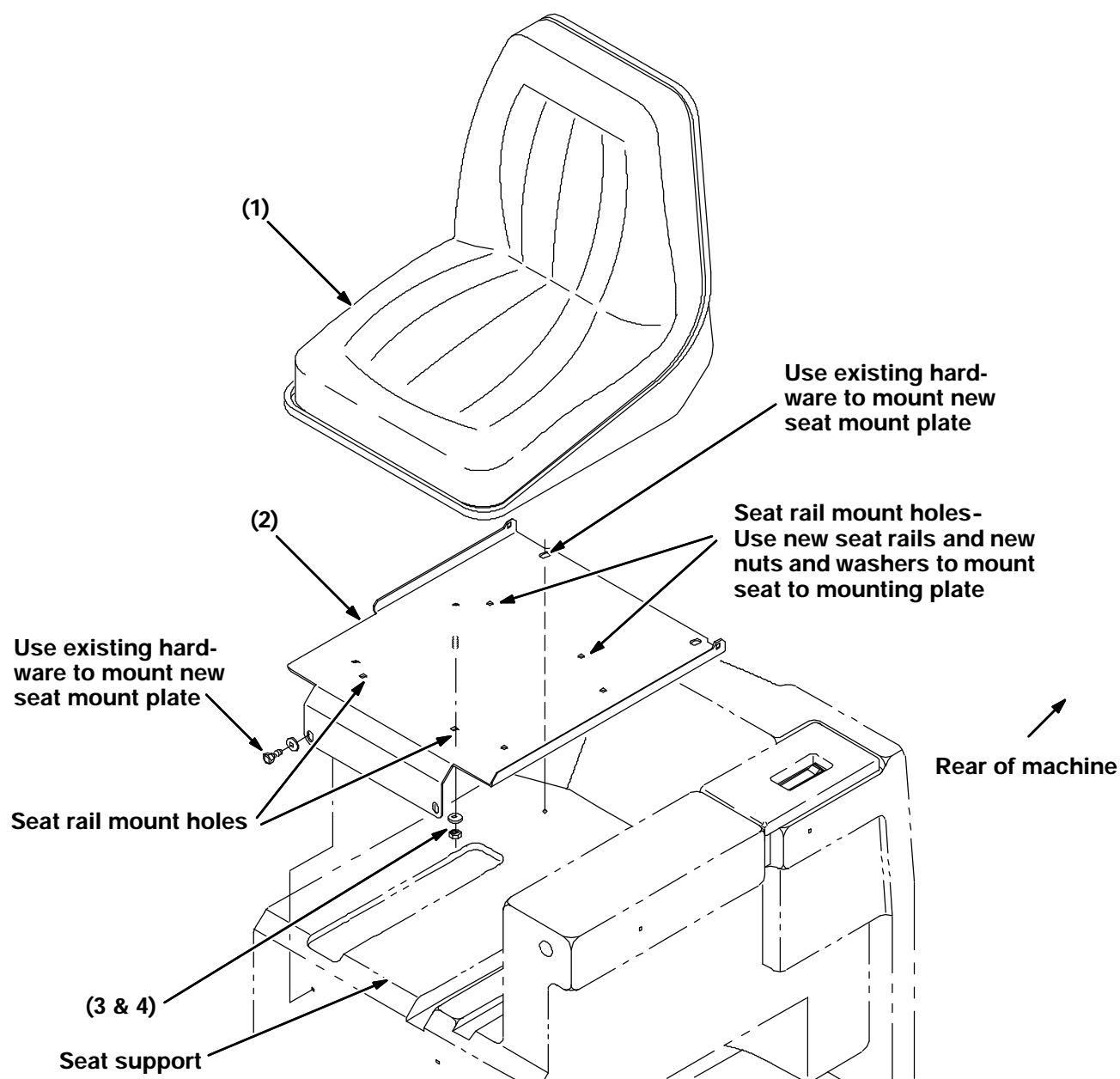
FIG. 1 - Installation of Michigan Seat Option
