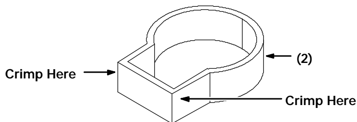
FIG. 1 - Crimping of Fuel Hose Clamp
