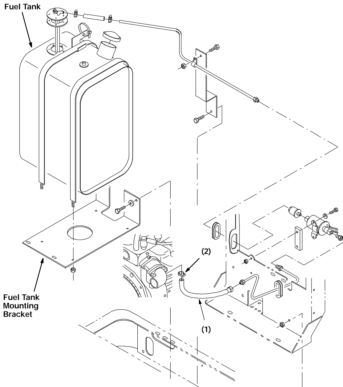
FIG. 2 - Installation of Replacement Fuel Hose
