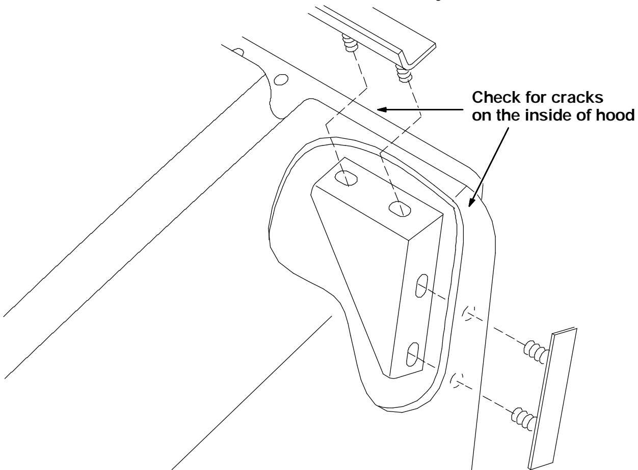
FIG. 2 - Corner Bracket Assembly
