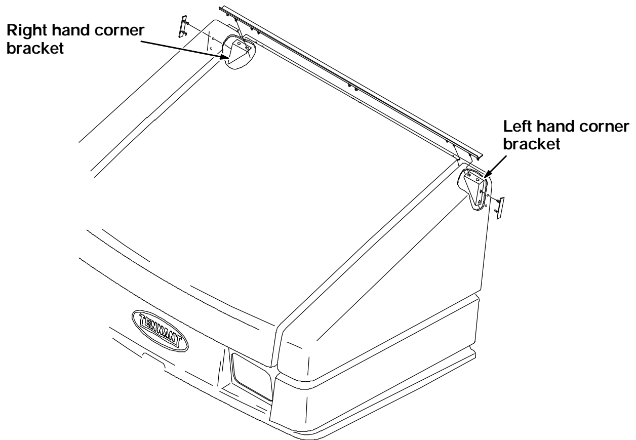
FIG. 1 - Hood Assembly
